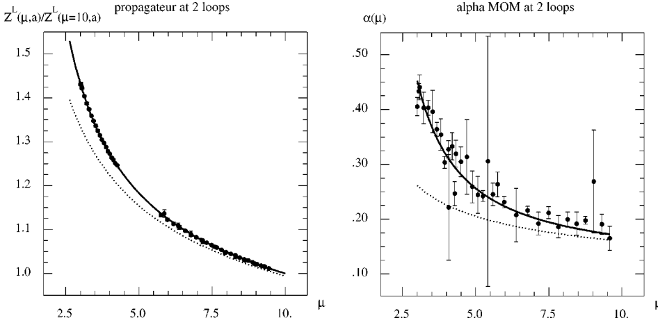
FIG. 2. Comparison of the two-loop fit to the ratio of the renormalization constants at k and at 10 GeV and to \alpha_s(k) with the lattice data for 2.5 < k < 10 GeV. The dotted line shows the perturbative part.
